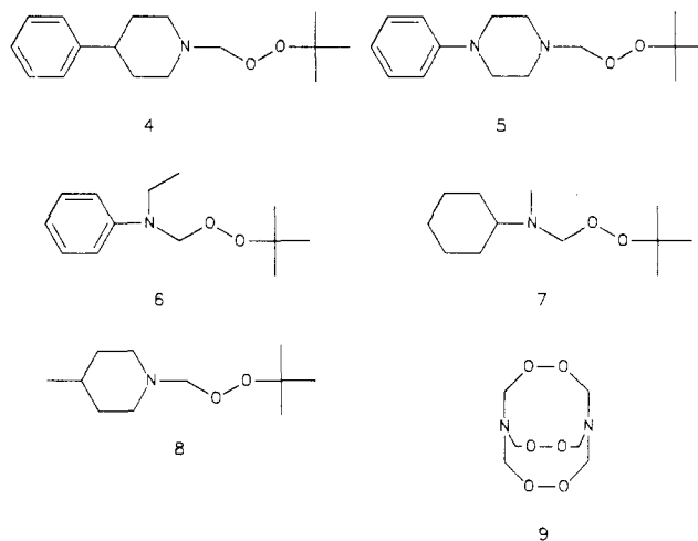
Figure 1. Structures of amine peroxides 4–9.
