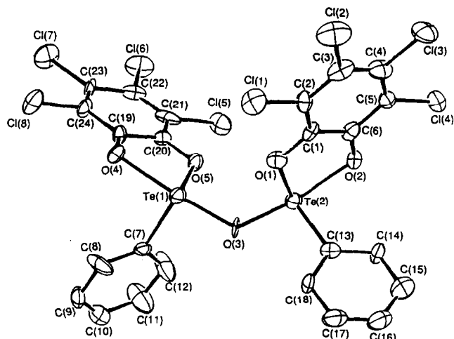
Fig. 1. The molecular structure of [(\text{Cl}_4\text{C}_6\text{O}_2)\text{Te}(\text{C}_6\text{H}_5)_2]_2\text{O} , shown as an ORTEP diagram, with 30% probability of ellipsoids. Hydrogen atoms have been omitted for clarity.
