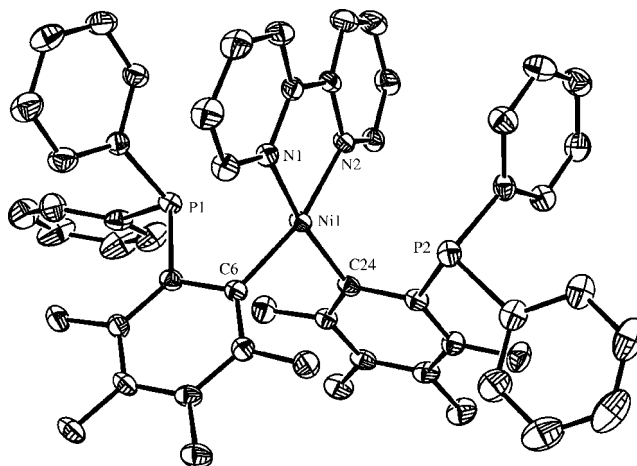
Figure 5. Molecular structure of cis - [\text{Ni}(\kappa\text{C-2-C}_6\text{F}_4\text{PPh}_2)_2(\text{bipy})] 9 . Ellipsoids show 30% probability levels, and hydrogen atoms have been omitted for clarity. Selected bond lengths (Å) and angles (deg): Ni(1)–N(1) 1.9489(19), Ni(1)–N(2) 1.9394(19), Ni(1)–C(6) 1.883(2), Ni(1)–C(24) 1.901(2), N(1)–Ni(1)–C(6) 95.18(9), N(2)–Ni(1)–C(24) 96.99(9), N(1)–Ni(1)–C(24) 166.28(9), N(2)–Ni(1)–C(6) 163.63(9), N(1)–Ni(1)–N(2) 82.79(8), C(6)–Ni(1)–C(24) 88.80(10).
