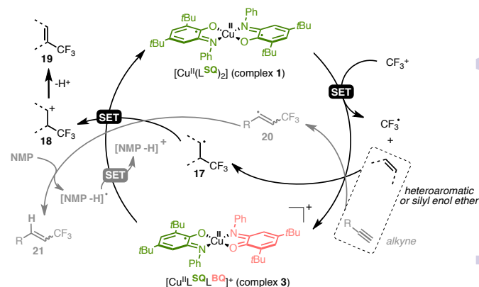
Scheme 2. Proposed mechanism for the controlled generation of CF 3 • radicals sustained by redox ligand. [NMP-H] • corresponds to the species resulting from H atom abstraction, more likely at the CH 2 position adjacent to the nitrogen.
