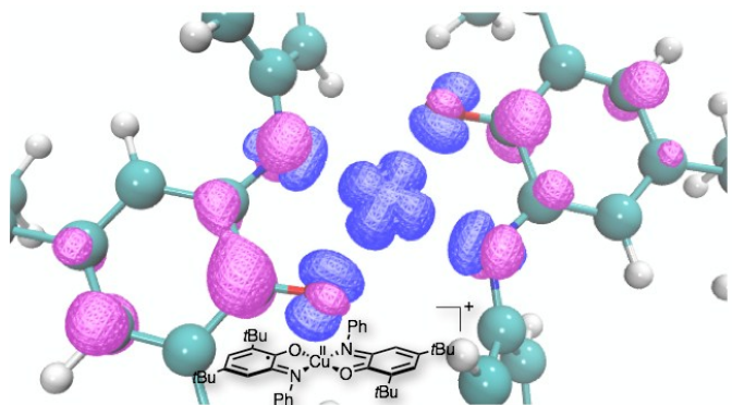
Figure 3. DFT optimized structure for complex 3 , together with a spin density isosurface (plotted at 0.005e/\text{\AA}^3 ).
