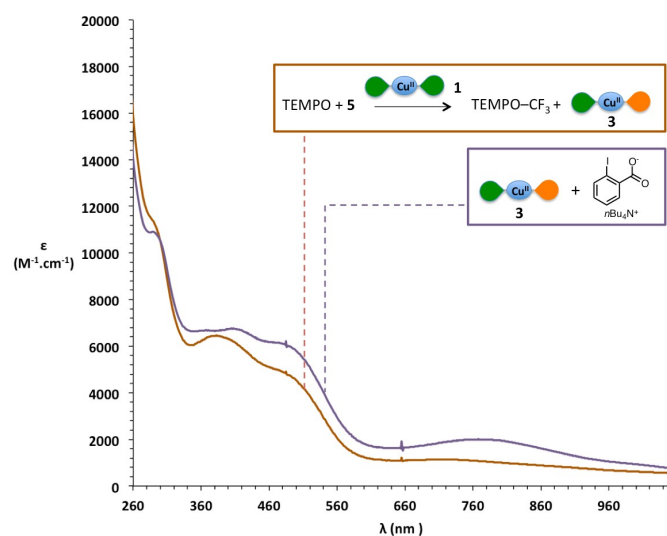
Figure 5. Comparison of UV-vis spectra in \text{CH}_2\text{Cl}_2 of: brick red : reaction with Togni II's source 5 ; purple : in situ generated [\text{Cu}(\text{L}^{\text{SQ}})(\text{L}^{\text{BQ}})]^+ 3 with added iodobenzoate. Color code for ligands: green petal is SQ ligand and orange petal is BQ ligand.
