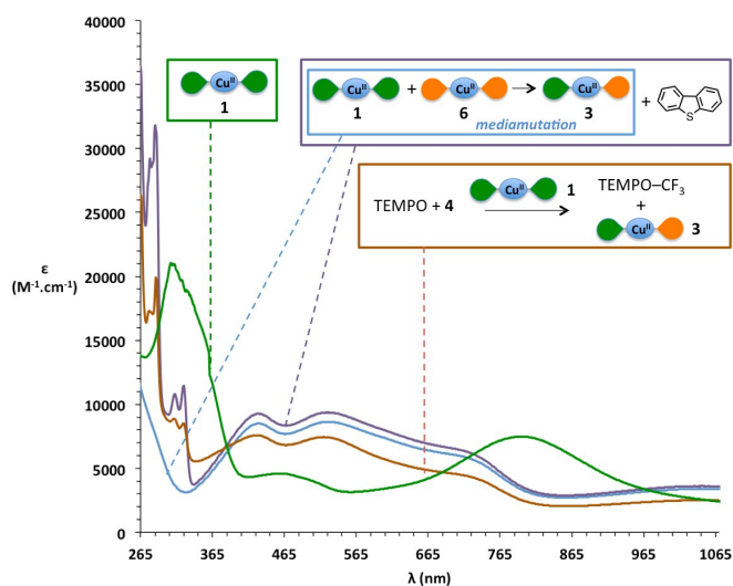
Figure 2. Comparison of UV-vis spectra in \text{CH}_2\text{Cl}_2 of: green : [\text{Cu}(\text{L}^{\text{SQ}})_2] 1 ; brick red : reaction with Umemoto's source 4 ; sky blue : in situ generated [\text{Cu}(\text{L}^{\text{SQ}})(\text{L}^{\text{BQ}})]^+ 3 ; purple : in situ generated [\text{Cu}(\text{L}^{\text{SQ}})(\text{L}^{\text{BQ}})]^+ 3 with added dibenzothiophene. Color code for ligands: green petal is SQ ligand and orange petal is BQ ligand.
