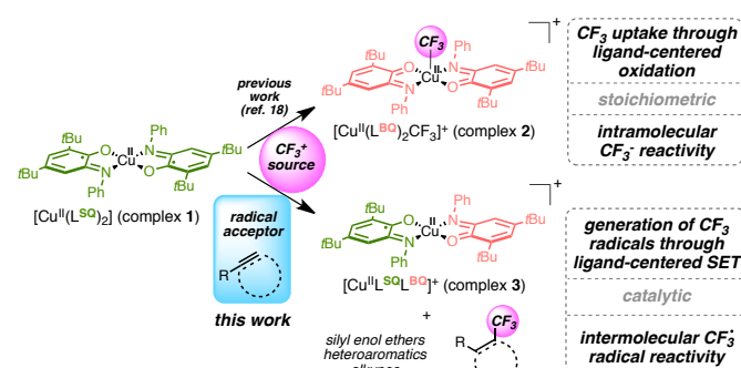
Figure 1. Ligand-based redox reactivity of complex 1 with an electrophilic CF 3 + source.
