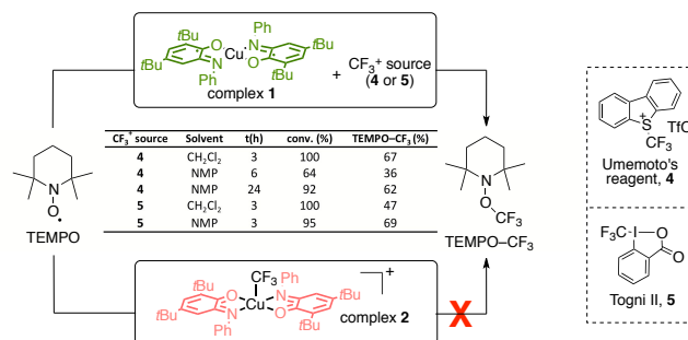
Scheme 1. TEMPO trapping experiments for the generation of \text{CF}_3 radicals with complexes 1 and 2 . NMP: N-methylpyrrolidinone.
