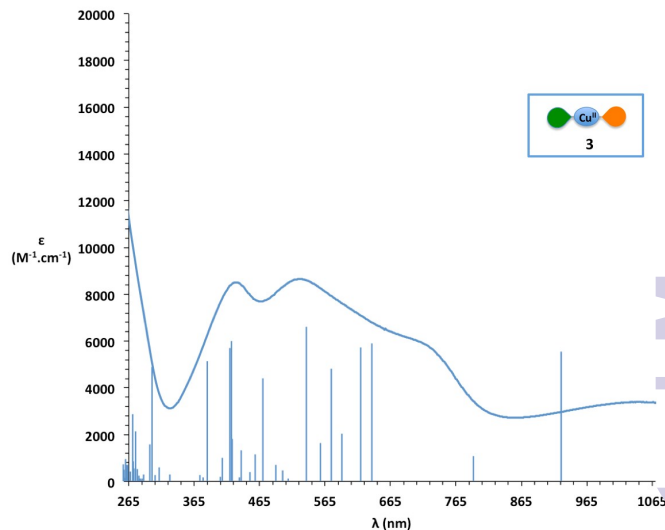
Figure 4. Comparison of DFT calculated peak positions (blue peaks) and experimental (blue curve) UV-vis spectrum of complex 3 .
