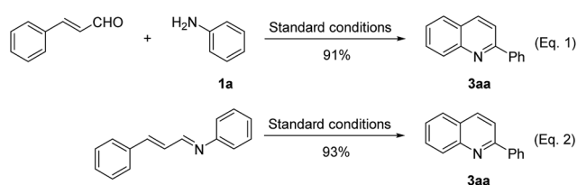
Scheme 2 Control experiments.
