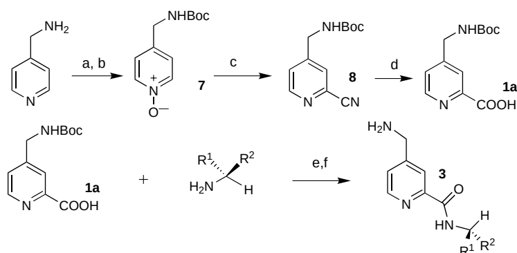
Scheme 2. Synthesis of the carrier 1a and the carrier/monoamine conjugate 3 . a) (Boc) 2 O, THF, TEA, room temperature, overnight (96 %); b) m CPBA, CH 2 Cl 2 , room temperature, 12 h (82 %); c) dimethylcarbamyil chloride, TMSCN, CH 2 Cl 2 , room temperature, 48 h (65 %); d) NaOH, EtOH(aq), reflux, 24 h (quant.); e) BOP, DIPEA, THF, room temperature, 4h; f) 10 % TFA/CH 2 Cl 2 , room temperature, 2 h (70–95 %).
