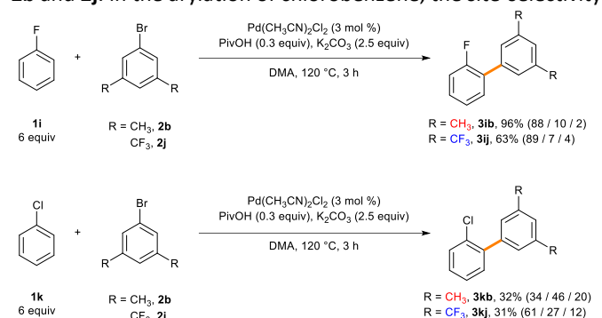
Scheme 5 C-H arylation of fluorobenzene and chlorobenzene with two different aryl bromides.
