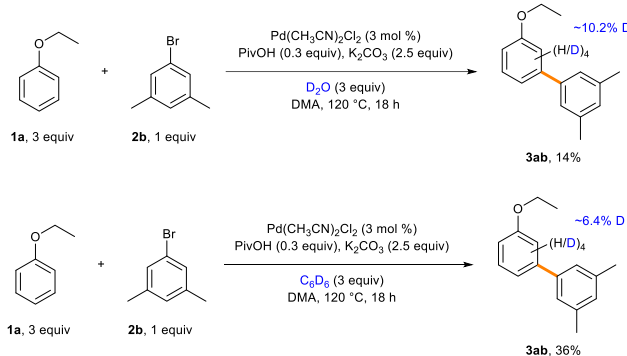
Scheme 6 Competition experiments.
