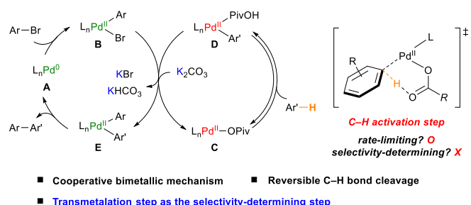
Scheme 1 Direct C-H arylation of simple arenes and selectivity.
