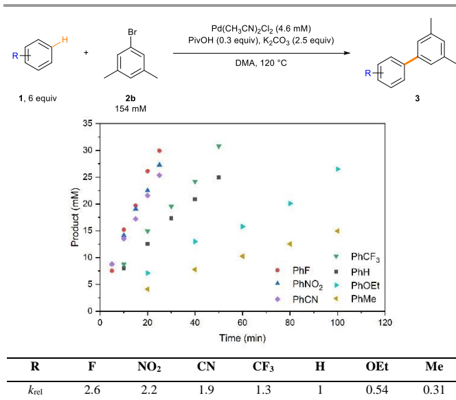
Scheme 2 Comparison of reaction rates. Combined yields of all isomers, determined by GC using dodecane as an internal standard, were used for kinetic plots. \sigma_p = Hammett constant. k rel = Relative reaction rate vs k (R=H) .
