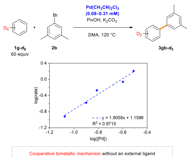
Scheme 4 Mechanistic hypothesis and kinetic studies.
