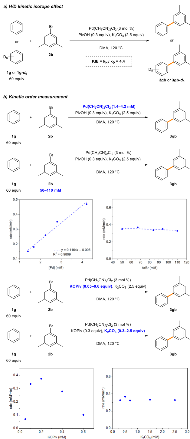
Scheme 3 Mechanistic studies.
