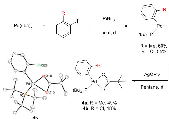
Scheme 7 Synthesis of arylpalladium pivalate complexes.
