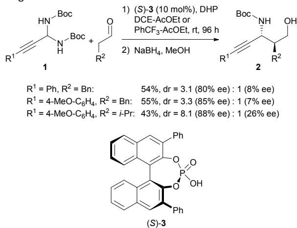
Scheme 2 Asymmetric Mannich reaction between N -Boc-aminals 1 and aldehydes.
