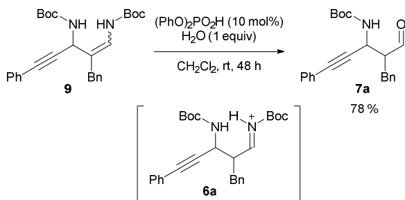
Scheme 5 Hydrolysis of enecarbamate 9 through iminium salt 6a .
