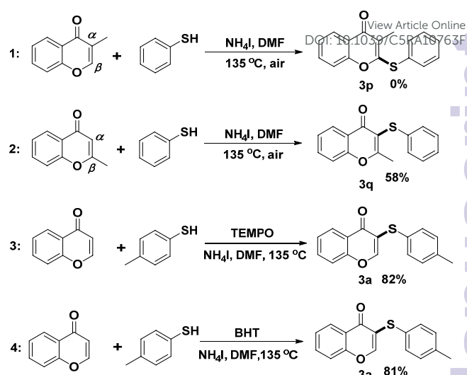
Scheme 2 Control reactions and radical trapping experiments.
