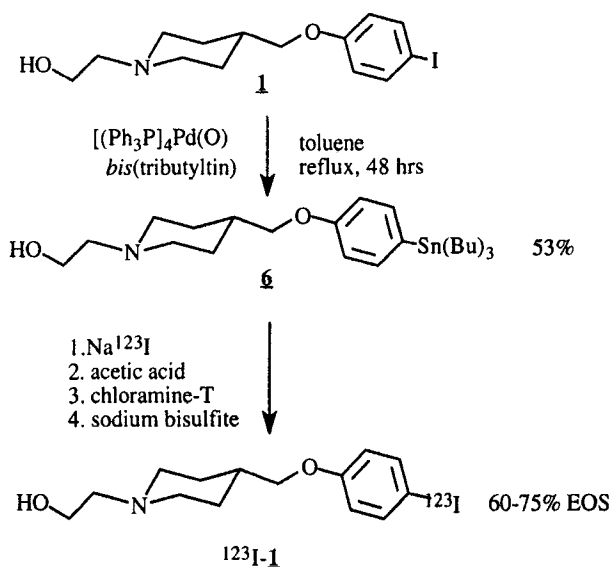
Scheme II. Preparation of ^{123}\text{I}-\mathbf{1} from 1 .
