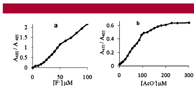
Figure 3. (a) Absorbance ratiometric (50 \mu M) responses ( A_{480}/A_{405} ) of chemosensor 2 and (b) 3 ( A_{475}/A_{405} ) upon incremental addition of fluoride and acetate ions respectively.
