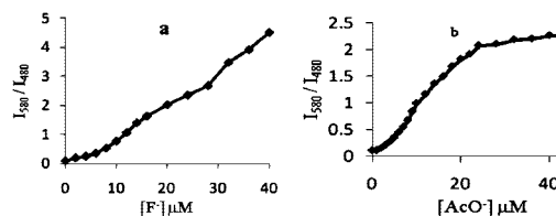
Figure 5. (a) Fluorescence ratiometric (10 \mu M) responses ( I_{580}/I_{480} ) of 2 and (b) 3 upon incremental addition of fluoride ions and acetate ions, respectively.
