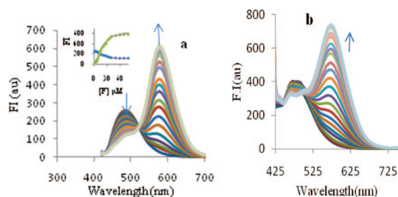
Figure 4. (a) Effect of incremental addition of fluoride ions on the fluorescence spectrum of 2 (10 \mu M) in CH 3 CN. Inset shows plot of fluorescence intensity versus [F − ] (points show the experimental results and line is curve fit). (b) Effect of incremental addition of acetate ions on fluorescence spectrum of 3 (10 \mu M) in CHCl 3 –MeOH (1:1).
