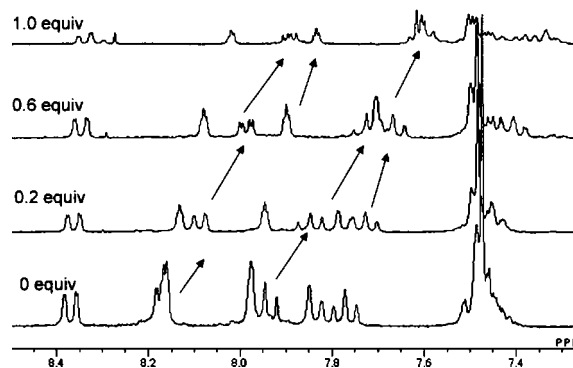
Figure 6. 1 H NMR spectra of chemosensor 2 on addition of TBA F in DMSO- d 6 .
