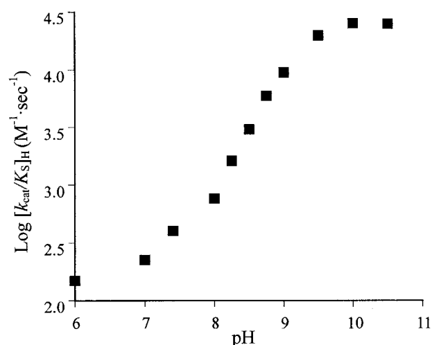
Fig. 2. Plots of [\log k_{\text{cat}}/K_S]_H against pH for the hydrolytic reaction of PNPA with HSA. Reaction conditions: 1/15 M phosphate buffer at 25°C. Plots represent mean \pm SD ( n = 3 ).
