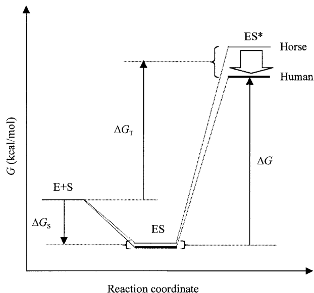
Fig. 3. Comparison of the free-energy profiles of the hydrolytic reaction of PNPA with albumin from human and horse. \Delta G_T , free-energy differences; \Delta G_S , free-energy change for the initial reaction of albumin and PNPA; \Delta G , activation free energy.
