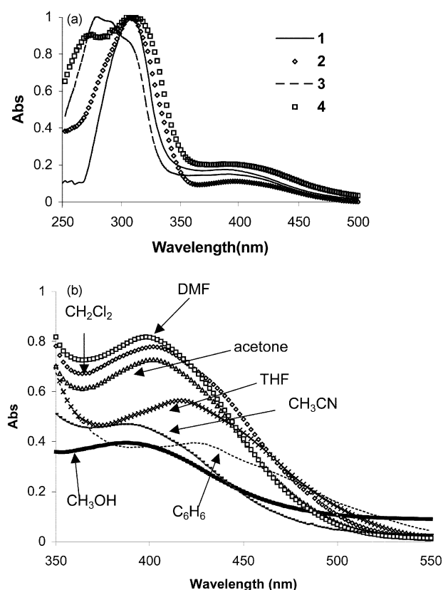
Fig. 5 Top: UV/Vis absorption spectra of complexes 1–4 in acetonitrile at 298 K. Bottom: UV/Vis spectra showing the MLCT band of 1 in various solvents at 298 K.
