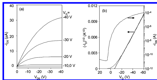
Figure 3. (a) Drain current I_{DS} versus source/drain voltage V_{DS} as a function of gate voltage V_G for an illustrative TFT with silver source/drain electrodes from the silver salt solution (channel length and width are, respectively, 25 and 1340\text{ }\mu\text{m} ). (b) I_{DS} and (-I_{DS})^{1/2} versus V_G at a constant V_{DS} = -60\text{ V} used for calculation of the mobility and current on/off ratio.
