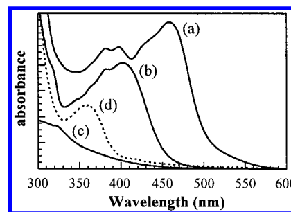
Figure 4. Electronic absorption spectra of (a) Ru 2 bpb, (b) Rebpb, (c) Rempb, and (d) bpb in acetonitrile. Spectra have been scaled in order to simplify their comparison. (Extinction coefficients are reported in Table 1).
