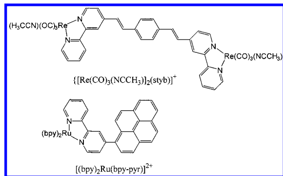
Figure 1. Complex structures from refs 6 and 9.
