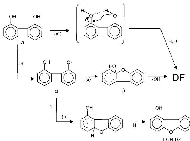
Scheme 4. Slow combustion of 2,2'-dihydroxybiphenyl ( A )
