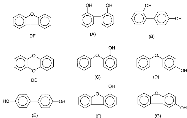
Figure 1. Structure of compounds; DF = dibenzofuran, DD = dibenzo- p -dioxin, A = 2,2'-dihydroxybiphenyl, B = 2,4'-dihydroxybiphenyl, C = 2-phenoxyphenol, D = 4-phenoxyphenol, E = 4,4'-dihydroxybiphenyl, F = 4-dibenzofuranol, and G = 2-dibenzofuranol.
