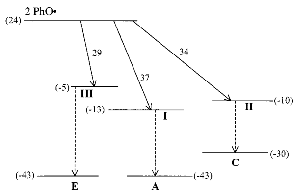
Figure 3. Enthalpy diagram (cf. Scheme 2)
