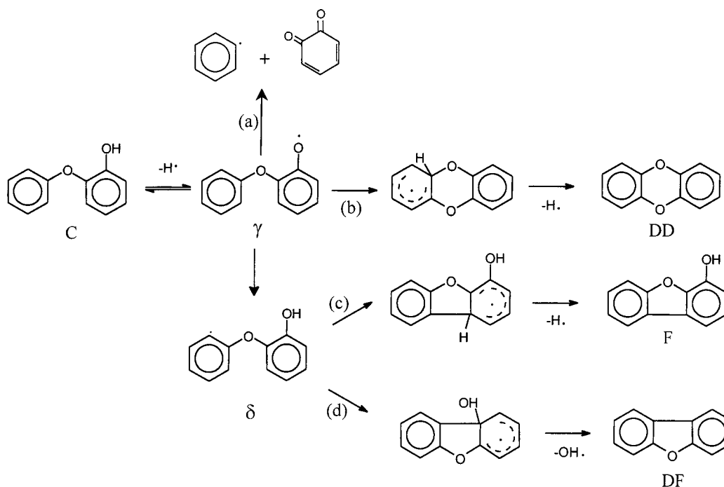
Scheme 3. Conversion of 2-phenoxyphenol ( C )
