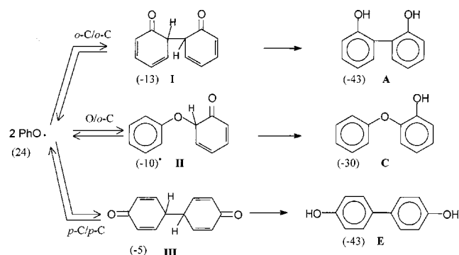
Scheme 2. Pathways for the condensation of phenoxy radicals
