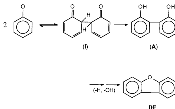
Scheme 1. Formation of dibenzofuran through the dimerisation of phenoxy radicals
