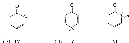
Figure 2. Structures of compounds IV , V , and VI
