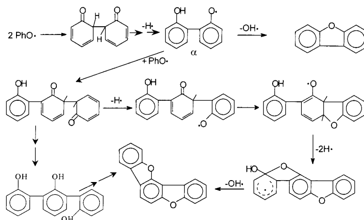
Scheme 5. Rationale for the formation of benzobisbenzofuran
