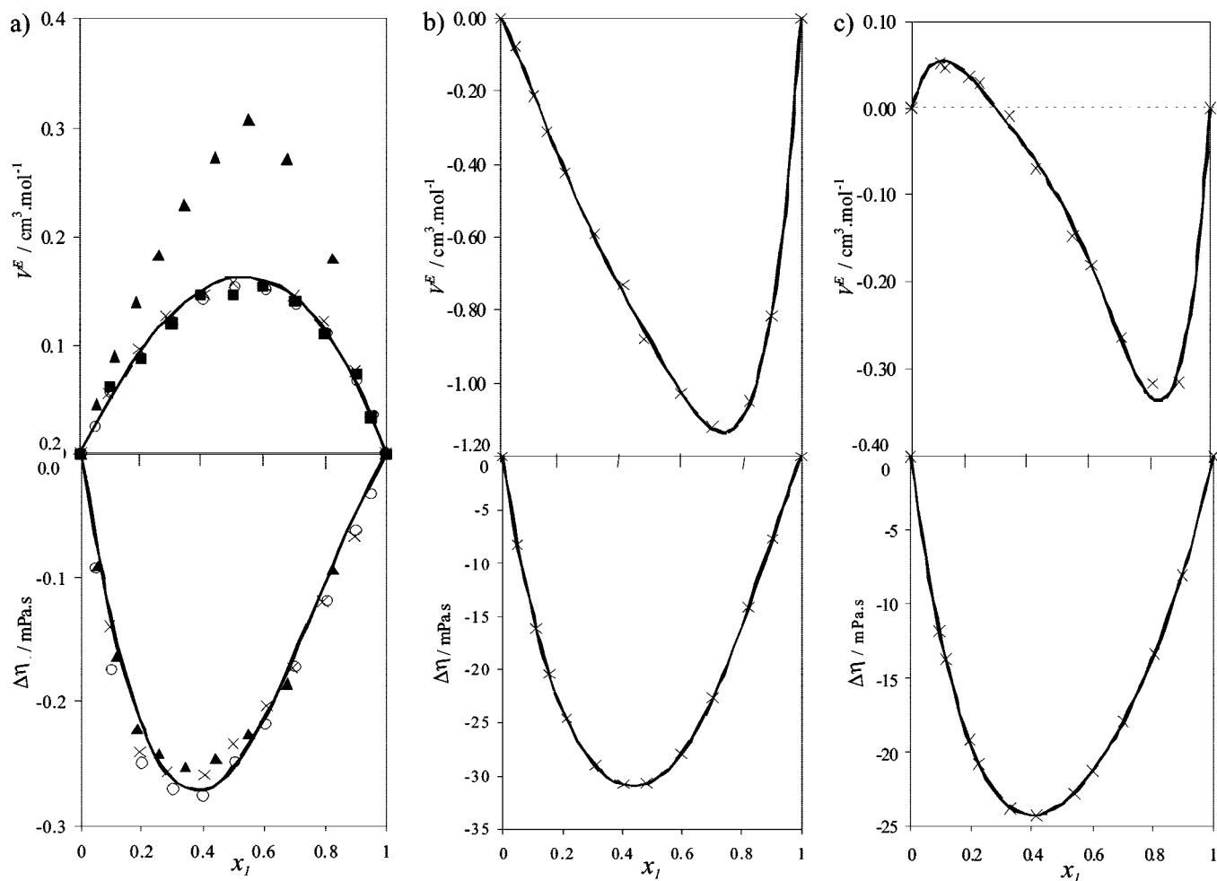
Figure 1. Excess molar volume and dynamic viscosity changes of mixing for binary systems at 298.15 K and atmospheric pressure: (a) ethyl acetate (1) + ethanol (2), (b) ethyl acetate (1) + [C 8 mim][NTf 2 ] (2), and (c) ethanol (1) + [C 8 mim][NTf 2 ] (2): x, this work; ■, ref 11; ○, ref 12; ▲, ref 13; —, Redlich–Kister correlation.
