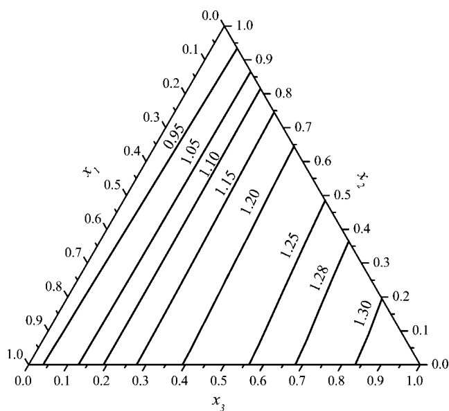
Figure 2. Density ( \text{g}\cdot\text{cm}^{-3} ) isolines for {ethyl acetate (1) + ethanol (2) + [C 8 mim][NTf 2 ] (3)} at 298.15 K and atmospheric pressure.
