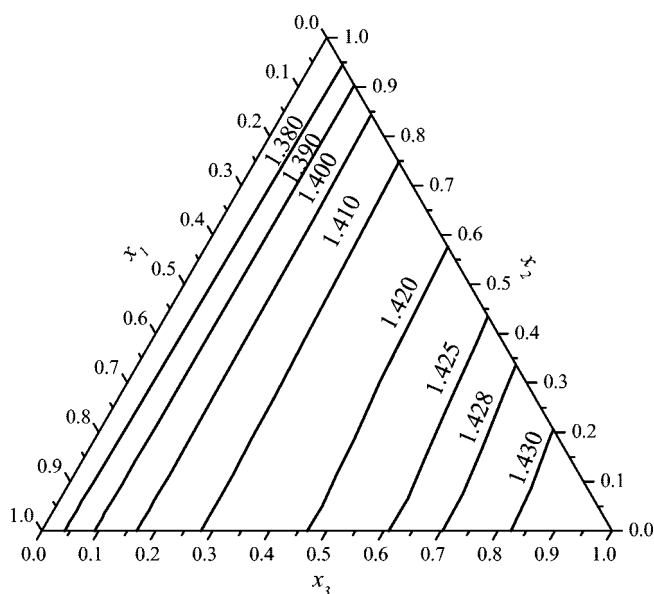
Figure 3. Refractive index isolines for {ethyl acetate (1) + ethanol (2) + [C 8 mim][NTf 2 ] (3)} at 298.15 K and atmospheric pressure.
