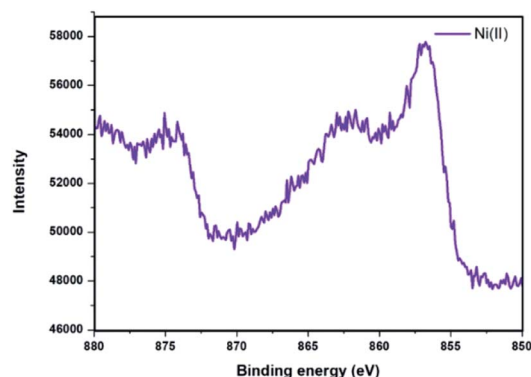
Fig. 5 XPS spectrum of \text{Ni@Fe}_3\text{O}_4\text{-C} catalyst.
