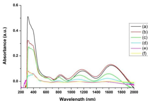
Figure 6: Electronic absorption of Cu-C2 films: (a) 5.68 \times 10^{-2} \text{ Ccm}^{-2} , (b) 4.35 \times 10^{-2} \text{ Ccm}^{-2} , (c) 2.38 \times 10^{-2} \text{ Ccm}^{-2} , (d) 5.80 \times 10^{-3} \text{ Ccm}^{-2} , (e) 2.94 \times 10^{-3} \text{ Ccm}^{-2} and (f) 2.30 \times 10^{-3} \text{ Ccm}^{-2}
