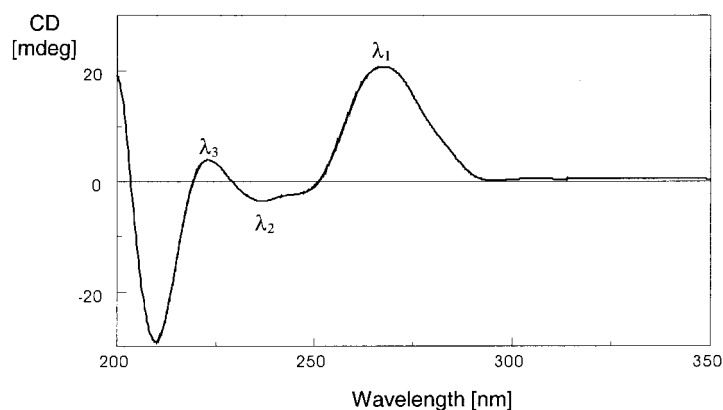
Fig. 5. Typical CD spectrum of a decamer hairpin loop
