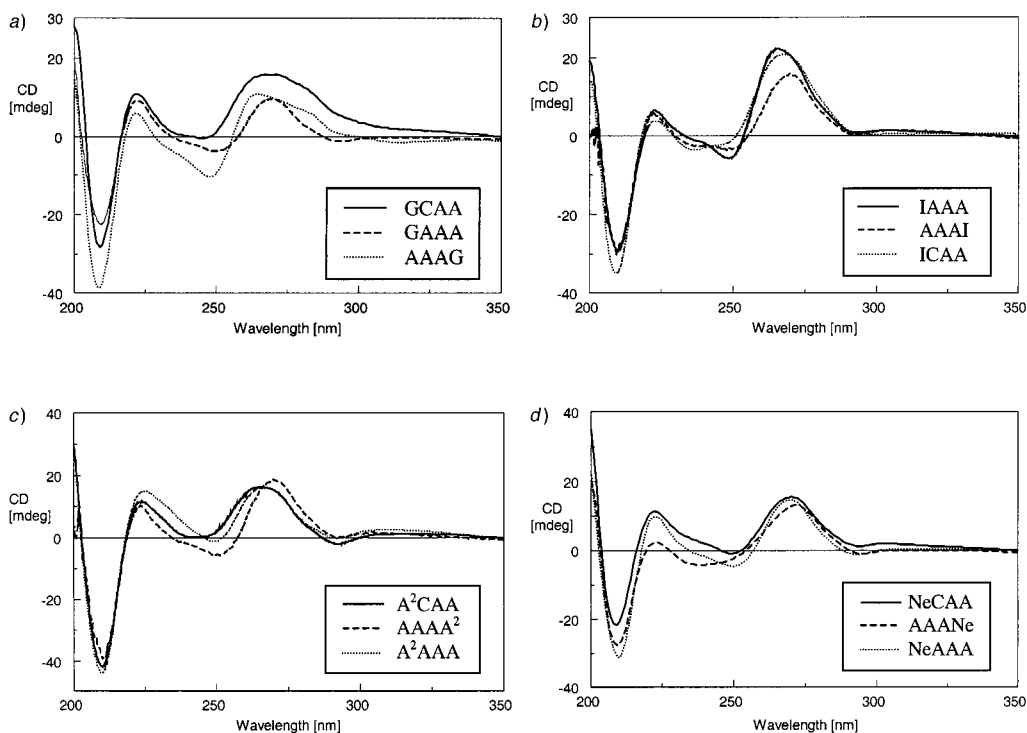
Fig. 6. CD Spectra of the synthesized decamer hairpins of the GNRA type: a) Changes in the loop sequence without modified bases; b) incorporation of inosine; c) incorporation of 9-( \beta -D-ribofuranosyl)-9H-purin-2-amine; d) incorporation of nebularine
