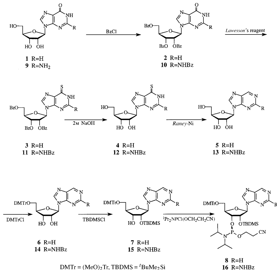
Scheme. Synthesis of the Nebularine and 9-( \beta -D-Ribofuranosyl)-9H-purin-2-amine Phosphoramidites 8 and 16 , Respectively
