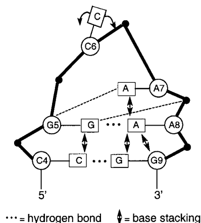
Fig. 1. Schematic representation of the GCAA loop with important structural features
