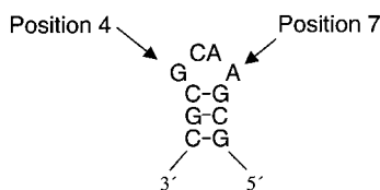
Fig. 4. Different base analogs were incorporated at position 4 and 7
