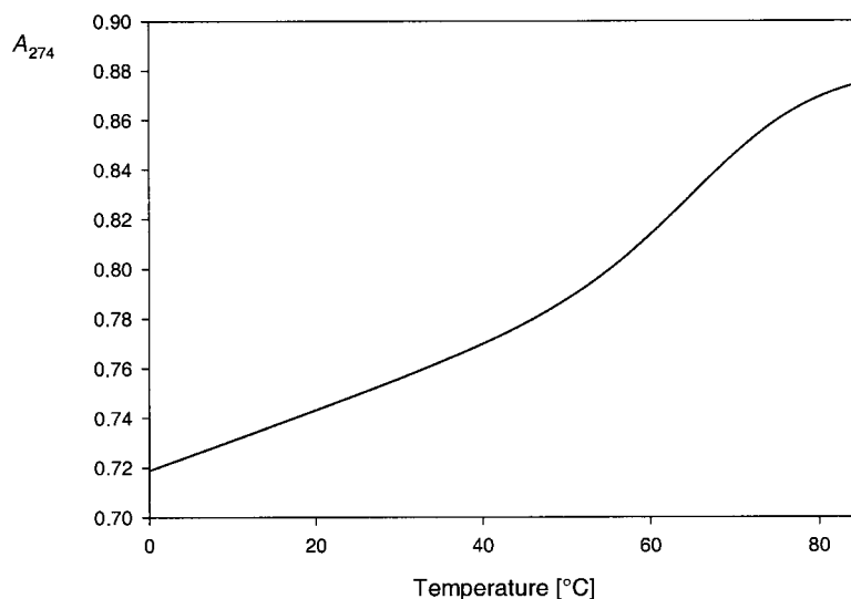
Fig. 3. Typical melting profile of a hairpin loop of the GNRA family (CGC-A 2 CAA-GCG)
