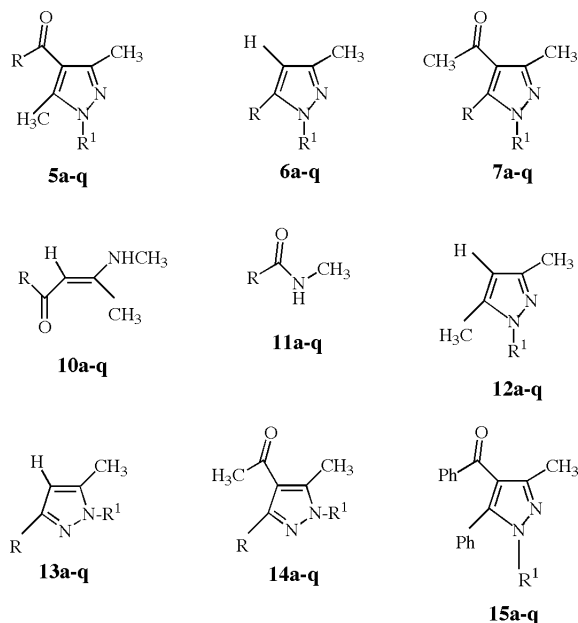
Figure 2. a) R = \text{CH(Ph)}_2 , R^1 = \text{CH}_3 ; b) R = \text{CH(CH}_3\text{)Ph} , R^1 = \text{CH}_3 ; c) R = \text{CH(CH}_3\text{)}_2 , R^1 = \text{CH}_3 ; d) R = \text{Ph} , R^1 = \text{CH}_3 ; e) R = \text{CH(Ph)}_2 , R^1 = \text{Ph} ; f) R = \text{CH(CH}_3\text{)Ph} , R^1 = \text{Ph} ; g) R = \text{CH(CH}_3\text{)}_2 , R^1 = \text{Ph} ; h) R = \text{Ph} , R^1 = \text{Ph} ; i) R = \text{CH(Ph)}_2 , R^1 = p\text{-Ph-NO}_2 ; j) R = \text{CH(CH}_3\text{)Ph} , R^1 = p\text{-Ph-NO}_2 ; l) R = \text{CH(CH}_3\text{)}_2 , R^1 = p\text{-Ph-NO}_2 ; m) R = \text{Ph} , R^1 = p\text{-Ph-NO}_2 ; n) R = \text{CH(Ph)}_2 , R^1 = \text{H(H}_2\text{O)} ; o) R = \text{CH(CH}_3\text{)Ph} , R^1 = \text{H(H}_2\text{O)} ; p) R = \text{CH(CH}_3\text{)}_2 , R^1 = \text{H(H}_2\text{O)} ; q) R = \text{Ph} , R^1 = \text{H(H}_2\text{O)} .
