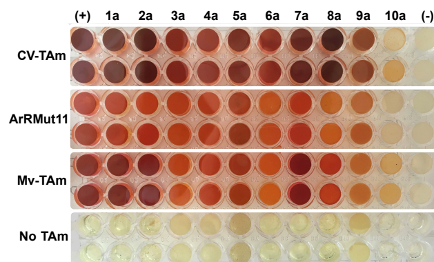
Figure 2 Colorimetric assay (in duplicate) using 2-(4-nitrophenyl)ethan-1-amine 12 as amine donor: 12 (25 mM), amino acceptor (10 mM), PLP (0.2 mM), KPi buffer pH 7.5 (100 mM) and enzyme crude lysate, 24 h, 30 °C, 500 rpm. Benzaldehyde was used as a positive control (+) and water as a negative control (-).
