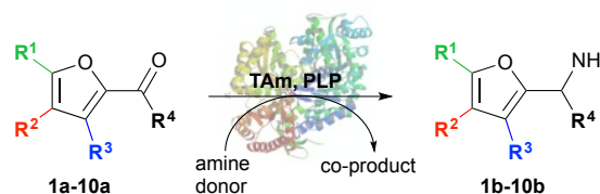
Scheme 1 Use of TAMs with co-factor pyridoxal-5-phosphate (PLP), aldehydes and ketone 1a-10a to generate amines 1b-10b .
