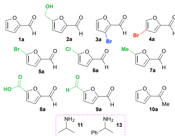
Figure 1 Furan-based substrates 1a-10a screened against TAmS, and amine donors IPA 11 and MBA 13 .
