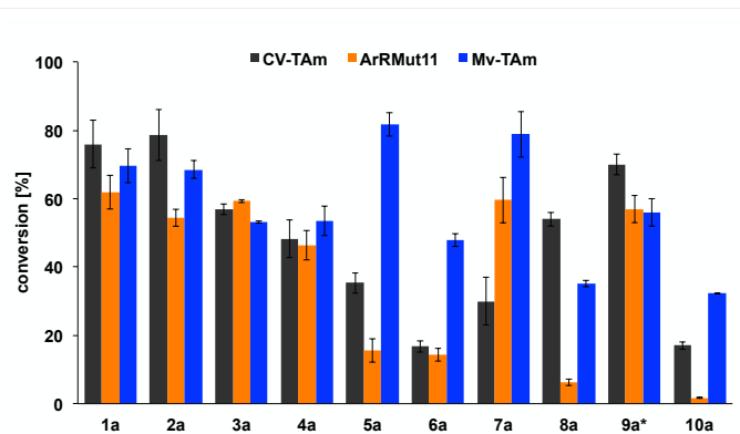
Figure 3 Screening results for substrates 1a–10a (5 mM) using 25 mM (S)- 13 (CV-TAM) or 25 mM (R)- 13 (ArRMut11 and Mv-TAM) as amine donors, 24 h, 30 °C. The product acetophenone was detected by HPLC analysis (at 254 nm) and used to determine % conversions. Background levels of acetophenone production were subtracted from the assay results in control reactions, and all reactions were performed in triplicate (standard deviations were less than 10%). Benzaldehyde (conversion of 68% with CV-TAM, 34% with ArRMut11, and 64% with Mv-TAM) was used as a positive control. *For 9a product formation was determined using a synthesised diamine standard 9b (see below).
