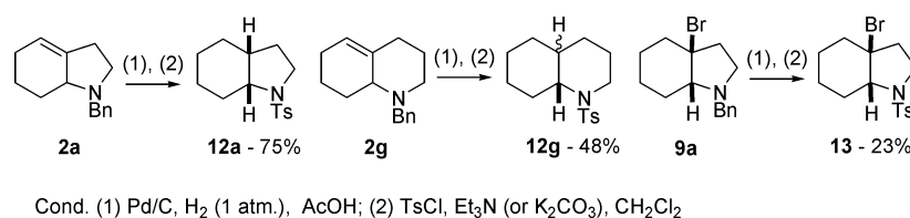
Scheme 6 Debenzylation of bicycles 2a , 2g and 9a .
