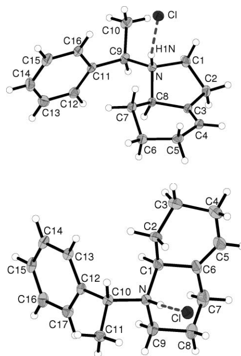
Fig. 1 X-ray crystallographic structures of ( R*,R* )- 2h ·HCl 12 and ( S,R )- 2i ·HCl 13 (thermal ellipsoids drawn at the 15% probability level). Note that for 2h ·HCl the co-crystallised H 2 O is not shown for clarity.
