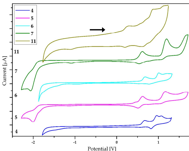
Figure 5 : CV curves of compounds 4-7 and 11 . Potentials are measured vs. Fc^+/Fc . The current of compound 11 was multiplied by the factor 10 to enhance visibility.
