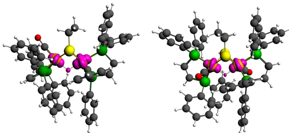
Figure 5. Unpaired spin density distribution in HFe 2 (pdt)(CO) 2 (dppv) 2 with isocontour plots at 0.005 e − /a 0 3 (violet). Atomic spin populations for unsym -[H1] 0 (left): Fe(1) 0.32, Fe(2) 0.64, H −0.03, P apical 0.053, P basal 0.001, −0.003, and −0.01. For sym -[H1] 0 (right): Fe 0.36 and 0.39, H −0.02, P apical 0.06 and 0.07, P basal 0.01 and 0.003.
