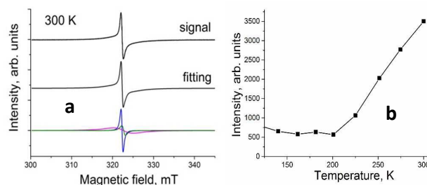
Fig. 5 EPR spectrum of 2 at 300 K (a). Temperature dependence of main component of EPR signal of salt 2 (b).
