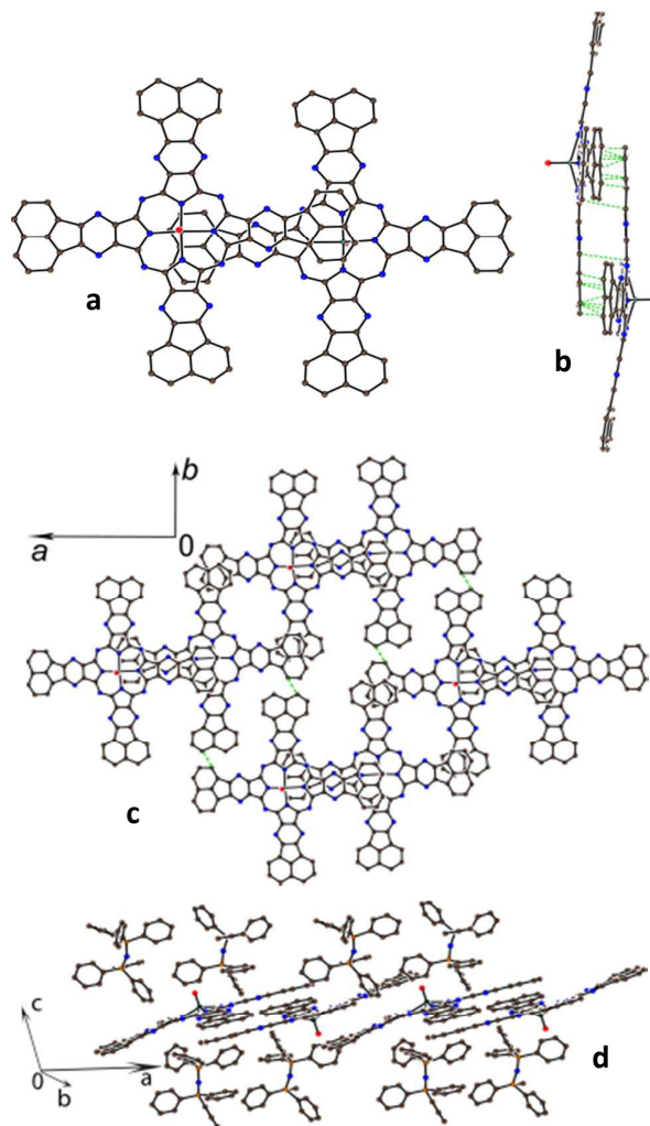
Fig. 4 Crystal structure of (PPN^+)_2[O=Ti^{IV}(AcTPzPz^{4-})]_2 \cdot 1.2C_6H_4Cl_2 \cdot 0.8C_6H_4Cl_2 ( 3 ): view on (a) and along (b) the \{[O=Ti^{IV}(AcTPzPz^{4-})]_2\}^{2-} dimer, view on (c) and along (d) the layers from the dimers. Shortened vdW C...C contacts are shown by green dashed lines. Solvent molecules are not shown for clarity.
