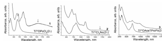
Fig. 1 UV-visible-NIR spectra of starting titanyl macrocycles and salts 1–3 in KBr pellets prepared in anaerobic conditions. Charge transfer bands (CTB) are shown by arrows.
