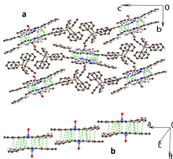
Fig. 3 Crystal structure of (PPN + ){O=Ti IV (Nc 3- )} 2- ·2C 6 H 4 Cl 2 ( 2 ). View along a axis and the naphthalocyanine chains (a) and view on these chains (b). Shortened vdW C...N...C, N...C, N contacts are shown by green dashed lines. Solvent molecules are not shown for clarity.
