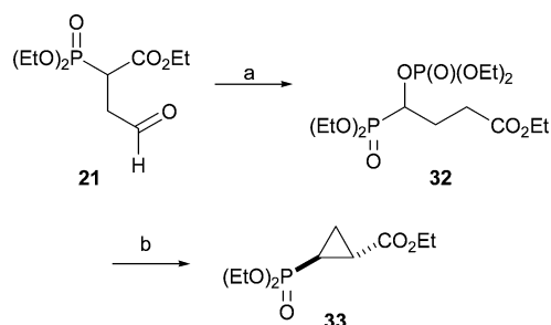
Scheme 8 Reagents and conditions: a) (\text{EtO})_2\text{P}(\text{OH})\text{H} , EtOH, EtONa (cat.), rt, 0.5 h; b) NaH, THF, reflux, 5 h.
