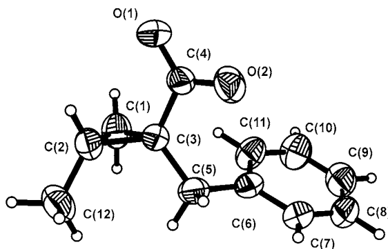
Fig. 2 The molecular structure of 1-benzyl-2-methylcyclopropanecarboxylate anion derived from the ester 7h .† In the crystal the anion is hydrogen-bonded to the dicyclohexylammonium cation. The latter has been removed from the plot for clarity. Displacement ellipsoids are drawn at the 50% probability level. H atoms are represented by circles of an arbitrary radius. The endocyclic cyclopropane bond lengths are: C1–C2 1.475(2), C2–C3 1.523(2), C1–C3 1.514(2) Å.
