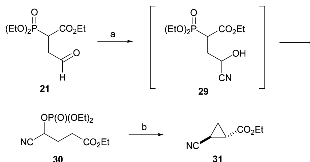
Scheme 7 Reagents and conditions: a) (\text{CH}_3)_2\text{C}(\text{OH})\text{CN} , \text{Ti}(\text{OiPr})_4 , r.t., 20 h; b) \text{NaH} , THF, reflux, 5 h.
