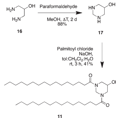
Scheme 1 Synthesis of cyclo -Pad-OH-Pad ( 11 ).
