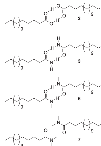
Fig. 1 Increasing intermolecular hydrogen bonding interactions leads to higher melting temperatures ( 2 to 3 ). The effect is reversed by blocking the hydrogen bond donating protons on the amide nitrogens ( 3 to 6 to 7 ).
