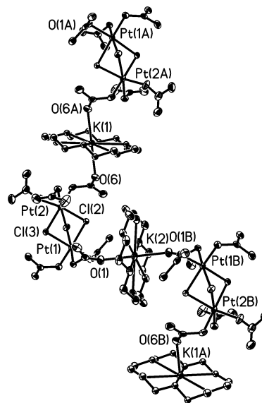
Figure 5. Ellipsoid representation of anions and cations in 1·C (50% probability). Selected K–O bond lengths (Å): K(1)–O(6) = 2.711(3), K(1)–O 18-C-6 (range) = 2.755(6)–2.825(9), K(2)–O(1) = 2.625(3), K(2)–O 18-C-6 (range) = 2.806(2)–2.841(3).
