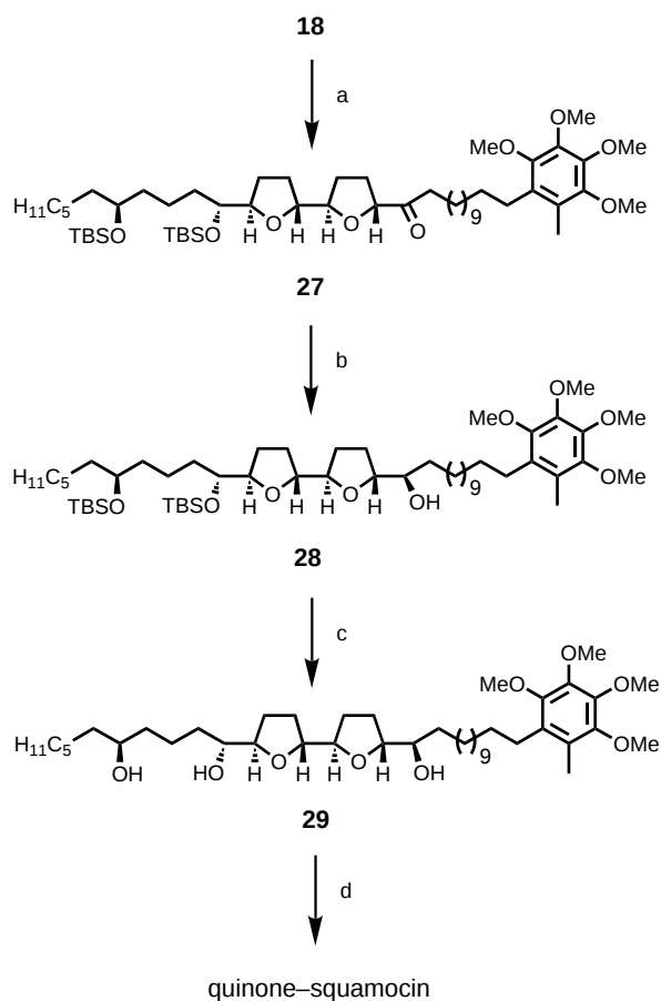
Scheme 9. Synthesis of quinone-squamocin D . a) 1) 18 (2.1 equiv), t BuLi (3.9 equiv), \text{Et}_2\text{O} , -105^\circ\text{C} , 4 min, \text{MgBr}_2 \cdot \text{OEt}_2 (4.9 equiv), -100 \rightarrow -40^\circ\text{C} , 1.5 h, -78^\circ\text{C} , 23 (1.0 equiv) \rightarrow 0^\circ\text{C} , 3.5 h, 52%, diastereomer ratio 1:1, 2.) (\text{COCl})_2 (75 equiv), DMSO (150 equiv), \text{NEt}_3 (250 equiv), \text{CH}_2\text{Cl}_2 , -40^\circ\text{C} , 1.5 h, 96%; b) L -selectride (15 equiv), THF, -70^\circ\text{C} , 1.5 h, 99%, diastereomer ratio 88:12, chromatographic separation of epimers; c) HF, \text{CH}_3\text{CN}/\text{CH}_2\text{Cl}_2 , 1.5 h, 77%; d) pyridine-2,6-dicarboxylic acid (6 equiv), CAN (12 equiv), \text{CH}_3\text{CN}/\text{H}_2\text{O} , 0 °C, 4 h, 70%. TBS = tert -butyldimethylsilyl.
