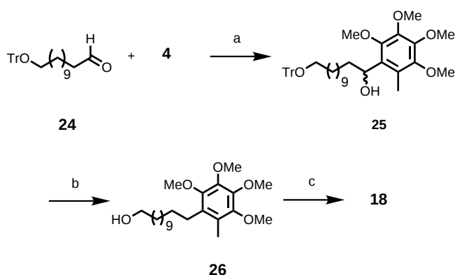
Scheme 8. Synthesis of iodide 18 . a) n BuLi (2.2 equiv), TMEDA, n -hexane, 0 °C, 2.5 h, 54%; b) \text{Et}_3\text{SiH} (5 equiv), \text{BF}_3 \cdot \text{OEt}_2 (7.5 equiv), \text{CH}_2\text{Cl}_2 , 14 h, 81%; c) imidazole (3 equiv), \text{PPh}_3 (1.1 equiv), \text{I}_2 (1.2 equiv) 0 °C, 4 h, 65%.
