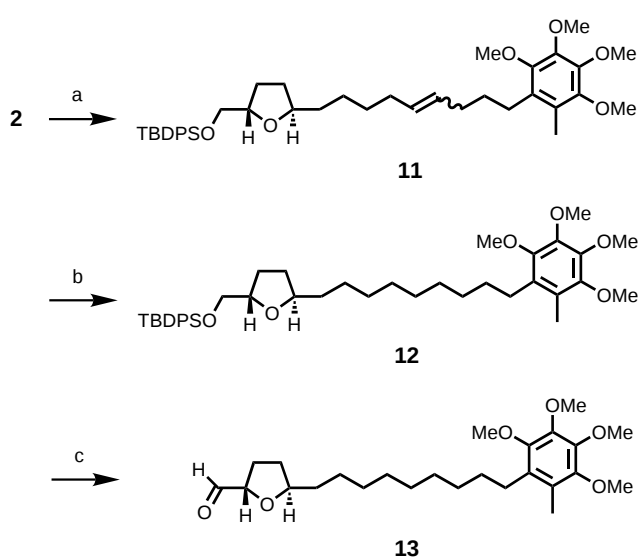
Scheme 4. Synthesis of aldehyde 13 . a) 2 (1.6 equiv), NaHMDS (1.1 equiv), THF, 0°C, 20 min, then 3 (1.0 equiv), 0°C, 1 h, 87%; b) Pt/C (0.02 equiv), H 2 , EtOAc, 6 h, 97%; c) 1.) TBAF (4.3 equiv), THF, 2.5 h, 95%; 2.) (COCl) 2 (2.0 equiv), DMSO (4.0 equiv), NEt 3 (5.0 equiv), CH 2 Cl 2 , –40°C, 1.5 h, 89%. TBAF = tetrabutylammonium fluoride, TBDPS = tert -butyldiphenylsilyl.
