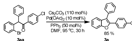
Scheme 4. Pd-catalyzed cyclization of intermediate 3aa
