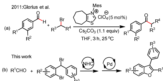
Scheme 2. Previous work and this work
