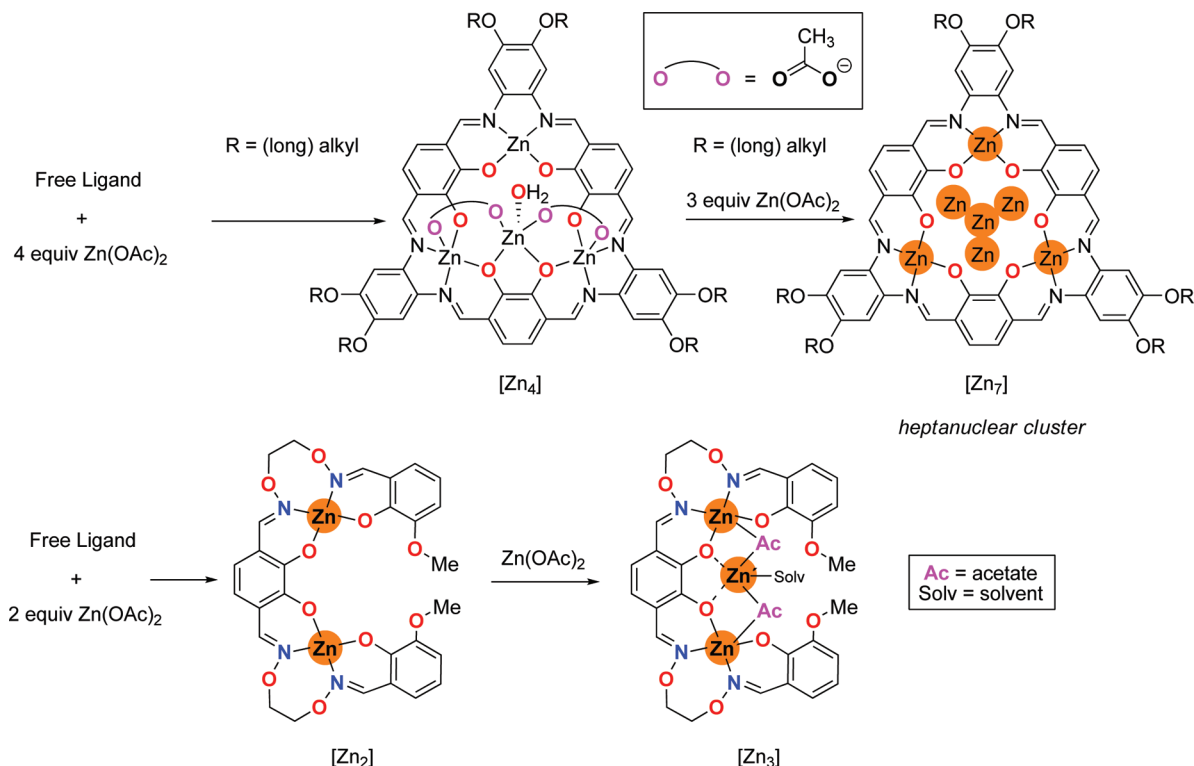
Figure 3. Schematic representation of the polynuclear salen complex formation reported by MacLachlan (at the top, [\text{Zn}_4] and [\text{Zn}_7] ) and Nabeshima (below, [\text{Zn}_2] and [\text{Zn}_3] ). Note the importance of both the array of internal O-donor atoms and the (bridging) acetate ligands.
