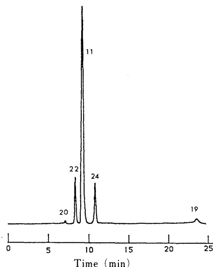
Fig. 3. HPLC Chromatogram of Products Obtained by Oxidative Coupling Reaction with Silver Oxide
