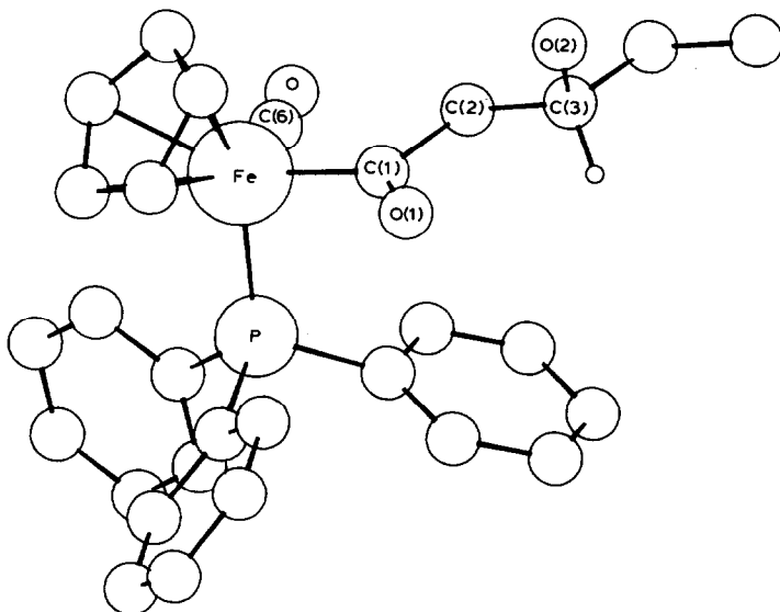
Fig. 1. Molecular structure of RR,SS-[(\eta^5-C_5H_5)Fe(CO)(PPh_3)(COCH_2CH(OH)CH_2CH_3)] ( 4b ).
