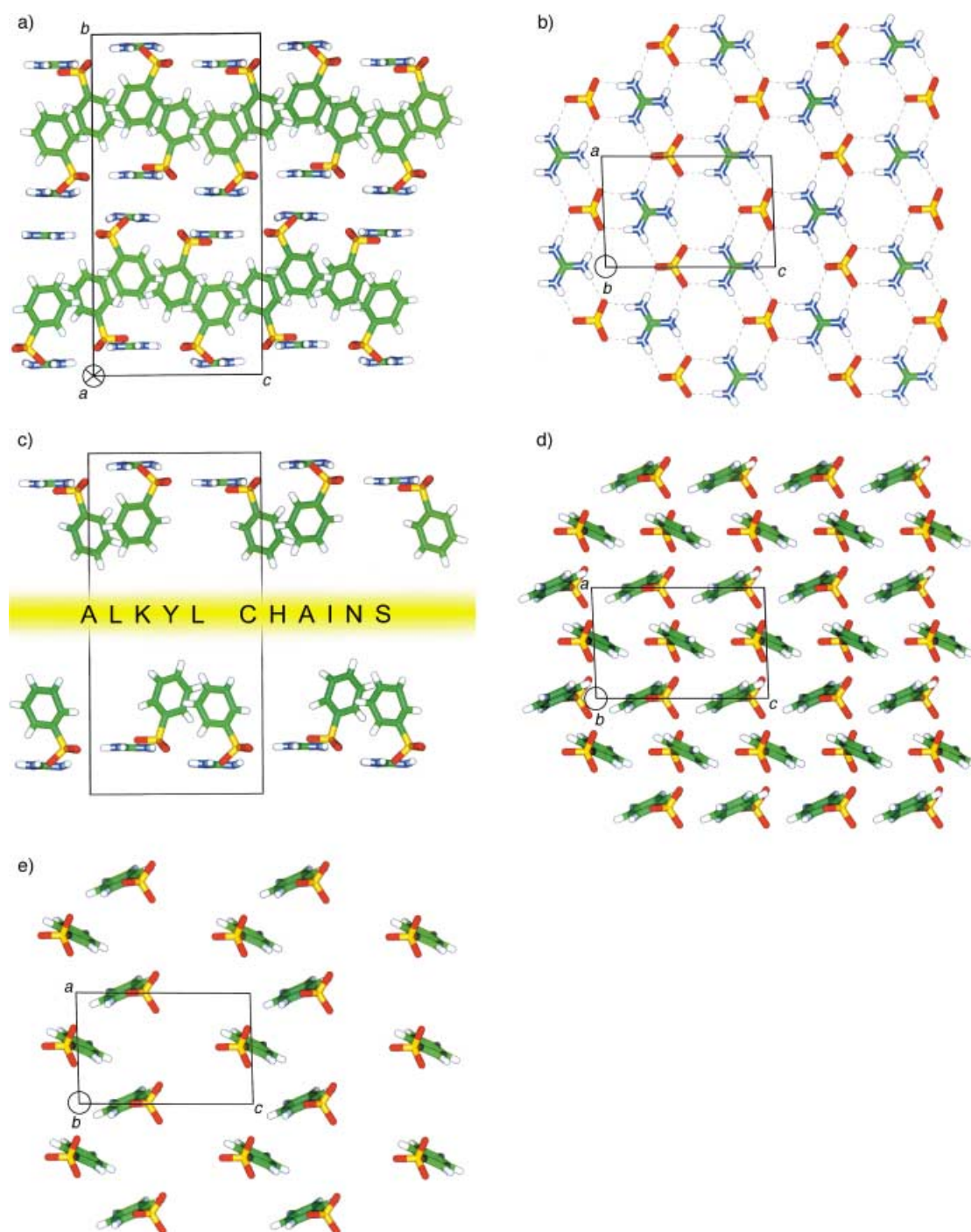
Figure 1. Crystal structure of guanidinium benzenesulfonate drawn by molecular modelling from experimental data of reference: [1] a) projection on b, c lattice plane of two layers of interdigitated molecules, b) packing mode in a, c lattice plane of sulfonate and guanidinium ions sitting on upper surface of upper molecular layer (benzene rings are omitted for clarity), c) splitting of the upper molecular layer, the molecules being drawn apart in order to leave enough space for the alkyl chains to be attached to the benzene rings, d) projection on a, c lattice plane of the upper layer of the interdigitated molecules (guanidinium ions are omitted for clarity), e) projection on a, c lattice plane of half the upper molecular layer (all guanidinium ions and molecules with sulfonate groups pointing downwards are omitted). Carbon atoms in green, sulphur atoms in yellow, oxygen atoms in red, nitrogen atoms in blue, hydrogen atoms in white. Cell parameters: a = 7.50 , b = 23.287 , c = 12.060 Å, \beta = 92.24^\circ .
