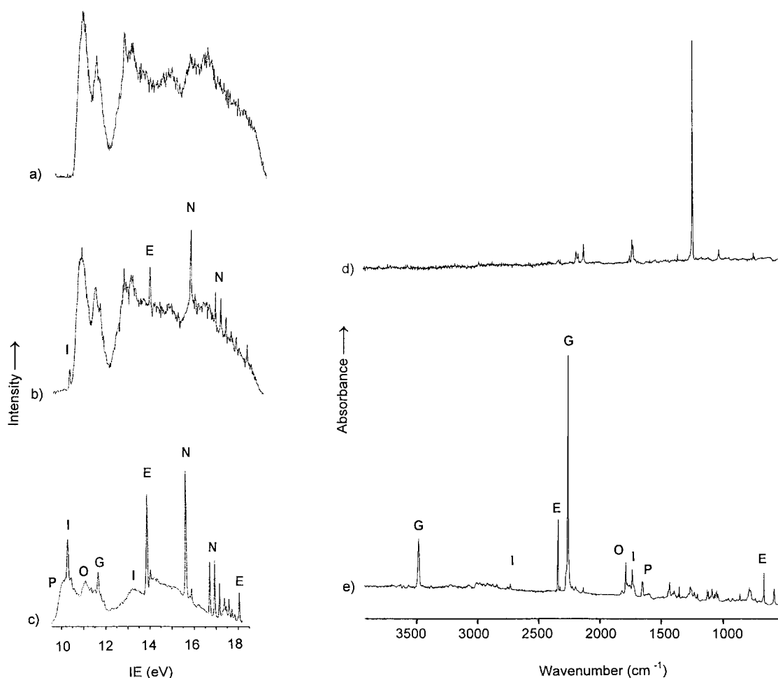
Figure 2. Spectra obtained during pyrolysis studies on \text{N}_3\text{COOEt} : a) PE spectrum of parent azide, before pyrolysis, b) PE spectrum after pyrolysis at about 190 °C, c) PE spectrum after pyrolysis at about 410 °C, d) \text{N}_2 matrix IR spectrum of parent azide, e) \text{N}_2 matrix IR spectrum after pyrolysis at about 280 °C.
