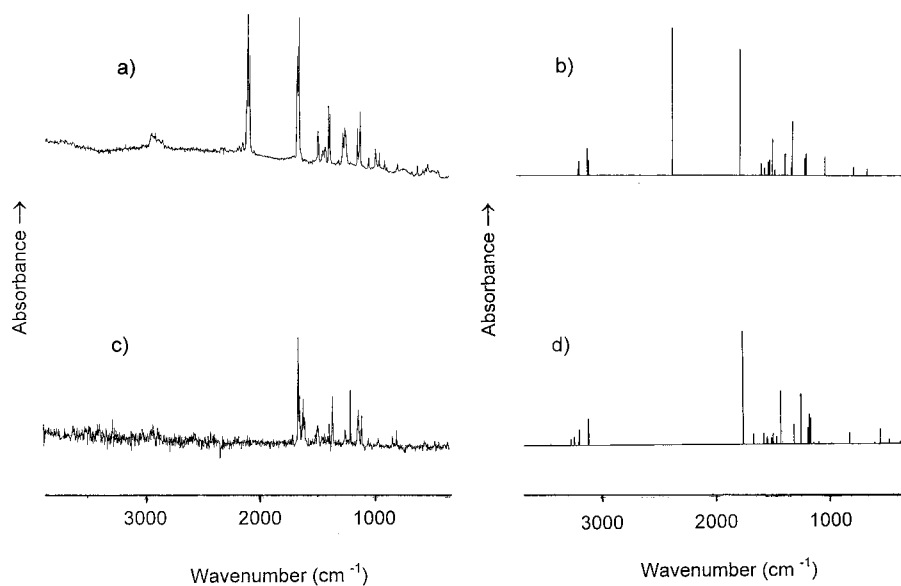
Figure 4. Comparison of observed and calculated IR spectra: a) observed spectrum of 2-azido- N,N -dimethylacetamide, b) calculated spectrum of 2-azido- N,N -dimethylacetamide, c) observed spectrum of iminodimethylacetamide, d) calculated spectrum of iminodimethylacetamide.
