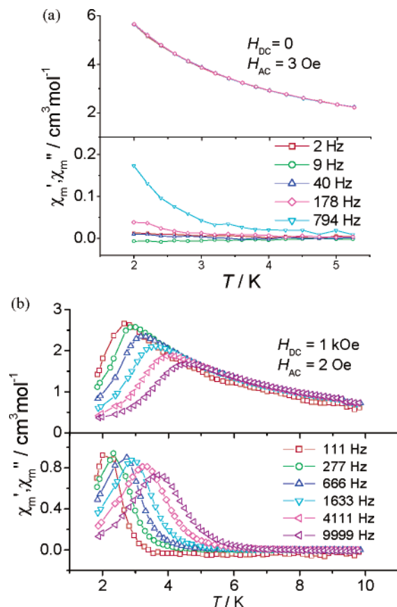
Figure 8. Plots of in-phase ( \chi_m' , top) and out-of-phase ( \chi_m'' , bottom) ac magnetic susceptibility versus temperature ( T ) for complex 4 : (a) under a zero dc field and (b) under a dc field of 1 kOe.
