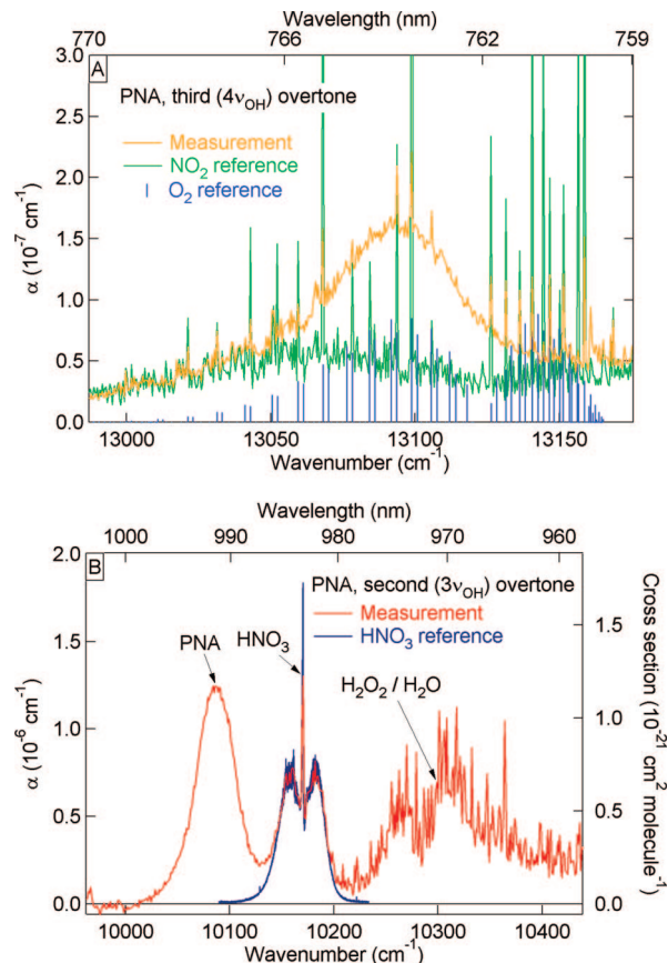
Figure 3. Cavity ring-down absorption coefficients \alpha , vs wavenumber (bottom) and wavelength (top); panel A: third ( 4\nu_{OH} ) overtone region of PNA with reference spectra of O 2 and NO 2 ; panel B: second ( 3\nu_{OH} ) overtone region of PNA, HNO 3 , and H 2 O 2 with reference spectrum of HNO 3 .
