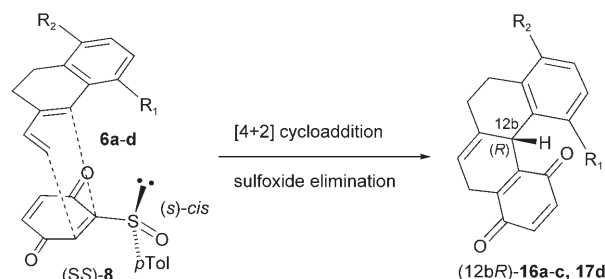
Scheme 14. Preferred approach between 3-vinyl-1,2-dihydronaphthalenes 6 and sulfinyl quinone (SS)- 8 .
