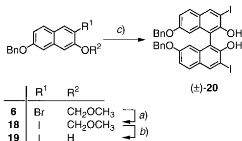
Scheme 3. Synthesis of (±)- 20
