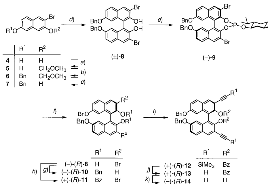
Scheme 1. Synthesis of the Macrocyclization Precursor (R)-13
