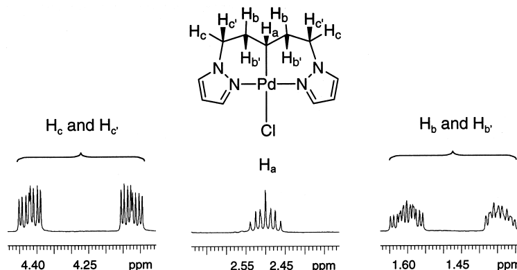
Fig. 1. Alkyl region of the ^1\text{H} -NMR spectrum for \text{Pd}\{\text{CH}(\text{CH}_2\text{CH}_2\text{pz})_2\text{-N,C,N'}\}\text{Cl} ( 6 ).
