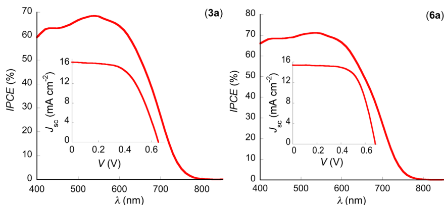
Figure 6. IPCE and photovoltaic (inset) data for 3a (left) and 6a (right).
