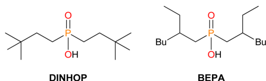
Figure 5. Chemical structures of bis(3,3-dimethyl-butyl)phosphinic acid (DINHOP) and bis(2-ethylhexyl)phosphinic acid (BEPA). It is shown that the latter acts as an effective coadsorbent in this study.
