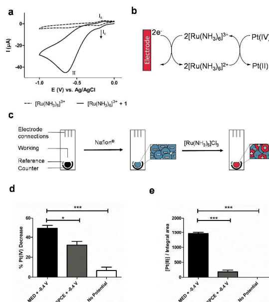
Fig. 1. (a) Overlay of the cyclic voltammograms of [Ru(NH 3 ) 6 ]Cl 3 (100 \mu M) in PBS (dashed line) alone, and following the addition of prodrug 1 (2 mM). A glassy carbon electrode was used as working electrode. Potentials are relative to the Ag/AgCl reference electrode employed. Processes ( I a ) and ( I c ) correspond to the reversible oxidation and reduction of the mediator, respectively, and ( II ) corresponds to the irreversible reduction of prodrug 1 (solid line); (b) Scheme showing the electro-catalytic mechanism for the reduction of the Pt(IV) prodrug 1 , where the ruthenium complex shuttles electrons from the electrode surface to the prodrug. The reduced ruthenium complex ([Ru(NH 3 ) 6 ] 2+ ) is electrochemically regenerated through the continuous application of the reduction potential characteristic for the redox couple [Ru(NH 3 ) 6 ] 3+ /[Ru(NH 3 ) 6 ] 2+ ; (c) The immobilisation of [Ru(NH 3 ) 6 ] 3+ onto the carbon ink screen-printed electrodes (SPCE) was carried out by coating the working electrode with the sulfonated fluoropolymer Nafion ® , followed by cation exchange entrapment of [Ru(NH 3 ) 6 ] 3+ . The successful entrapment of the redox mediator was confirmed by CV analysis in PBS with the immobilised [Ru(NH 3 ) 6 ] 3+ showing the expected reversible redox behaviour (Fig. S4, ESI † ); (d) and (e) Electroactivation of prodrug 1 by the application of -0.4 V with modified electrode (MED) or un-modified electrode (SPCE) in PBS with HPLC monitoring of: (d) %Pt(IV) and (e) the Pt(II)-GMP bisadduct ( n = 3). The data represent the mean \pm S.D. *** P < 0.001 by one-way ANOVA with Tukey post-test.
