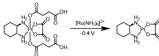
Scheme 1 Prodrug 1 electrochemically activated to the active anti-cancer drug oxaliplatin, 2 mediated through electron transfer by [\text{Ru}(\text{NH}_3)_6]^{2+} .
