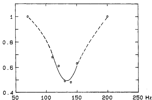
Fig. 1. Saturation-transfer effect for H\text{--C}(8) of (+)- 1 . Abscissa: upfield shift in Hz of the decoupler frequency with respect to the H\text{--C}(8) frequency of conformer 1a ( = 0 Hz). Ordinate: resulting effect from the unperturbed signal area (1) to the maximum effect (ca. 0.5).
