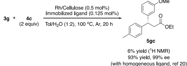
Scheme 4 Reaction with the mixture of Rh NPs and chiral ligand on different supports
