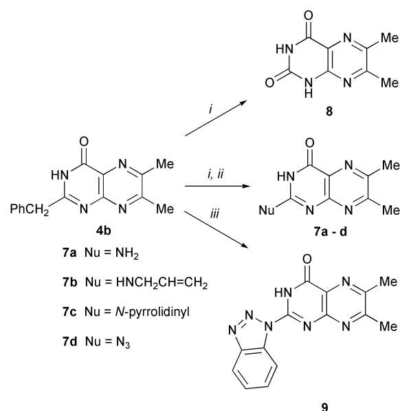
Scheme 2 Reagents: i aq. DDO; ii DDO followed by Nu; iii N -chlorobenzotriazole.
