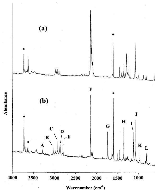
Figure 1. Nitrogen matrix infrared bands observed during pyrolysis studies on 2-azidoethanol. Absorptions denoted by an asterisk are assigned to \text{H}_2\text{O} . Band identification is shown in Table 1. Spectrum a was obtained with no superheating (parent 2-azidoethanol sublimed at room temperature). Spectrum b was obtained after passage through superheater at 570 °C.
