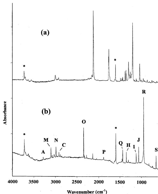
Figure 3. Nitrogen matrix infrared bands observed during pyrolysis studies on 2-azidoethyl acetate. Absorptions denoted by an asterisk are assigned to \text{H}_2\text{O} . Band identification is shown in Table 1. Spectrum a was obtained with no superheating (parent ester sublimed at room temperature). Spectrum b was obtained after passage through superheater at \sim 500^\circ\text{C} .
