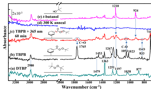
Fig. 2 RAIR spectra of (a) DTBP dosed on SLG/Cu at 120 K, (b) 0.1 L TBPB dosed on SLG/Cu at 200 K, (c) sample (b) after 60 minutes UV irradiation, (d) sample (c) following vacuum annealing to 300 K, and (e) t -butanol dosed on SLG/Cu at 120 K. The drawings serve to assist in vibration mode assignments; no molecular-level structural details are implied.
