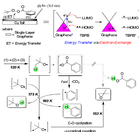
Fig. 4 Proposed reaction mechanism.
