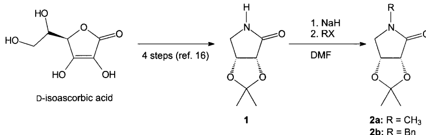
Scheme 3. Synthesis of the sugar lactams 2a,b .
