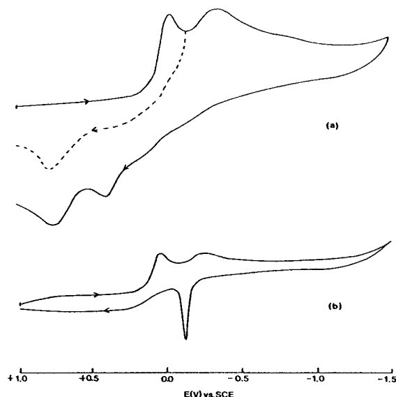
Figure 4. Cyclic voltammograms in the scan range +1.0 to -1.5 V for Cu 2 (stz) 4 in acetone solution (a) at a scan rate of 0.15 V·s -1 and in acetonitrile solution (b) at a scan rate of 0.05 V·s -1 .
